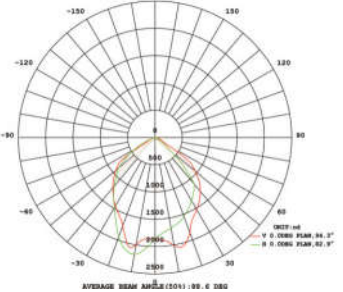
Luminous Intensity Distribution Curve 配光曲线
