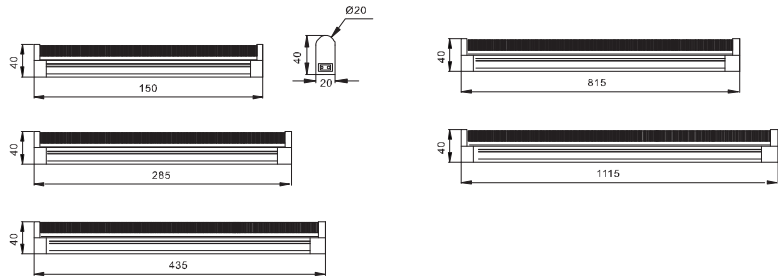
Adjustable T4 LED Fixture 可调角度T4 LED支架
