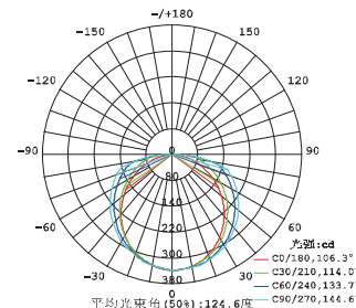
Luminous Intensity Distribution Curve 配光曲线
