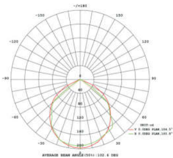
Luminous Intensity Distribution Curve 配光曲线
