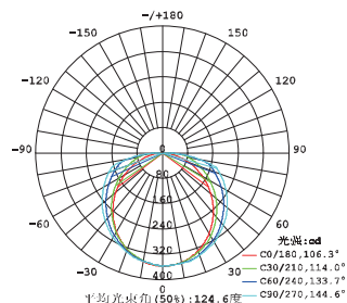
Luminous Intensity Distribution Curve 配光曲线
