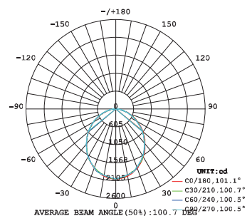
Luminous Intensity Distribution Curve 配光曲线
