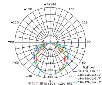
Luminous Intensity Distribution Curve 配光曲线
