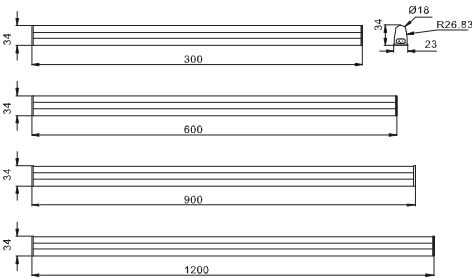
T5 LED Integrated Fixture / T5 LED一体化支架
